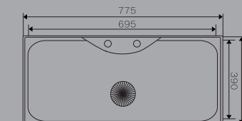
ITEM NO.:XL-132-1 ANAL YSIS SIZE:775*475 SURAF CCE Satin/Polish/Ele-pearl/Dekor/Linen
