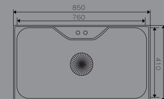
ITEM NO.:XL-132 ANAL YSIS SIZE:850*500 SURAF CCE Satin/Polish/Ele-pearl/Dekor/Linen
